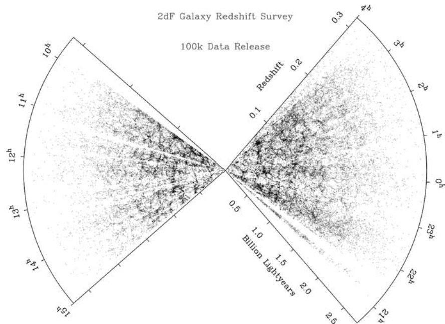
FIGURE 13-28 The 2dF Galaxy Redshift Survey (2dFGRS) is a major spectroscopic survey utilizing unique facilities built by the Anglo-Australian Observatory. By the survey’s completion in 2002, it had recorded precise spectra for 245,591 objects making possible a wide range of new analyses, including, for example, the first direct comparison with the microwave background anisotropy on the same spatial scale and studies of galaxy clustering to test inflationary cosmological models of the early universe. The survey is integrated with the 2dF Quasi Stellar Objects survey. [Matthew Colless and the 2dF Galaxy Redshift Survey Team.]
